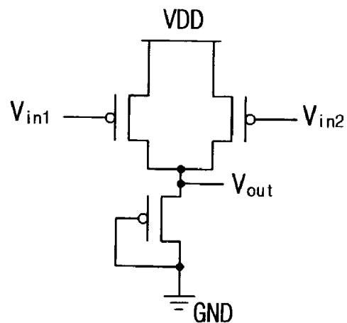
<NAND GATE>
