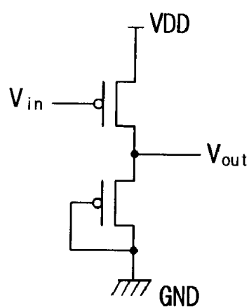
<INVERTER>
