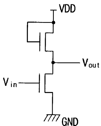
<INVERTER>
