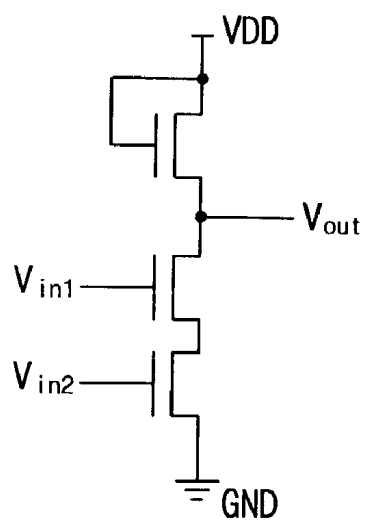
<NAND GATE>
